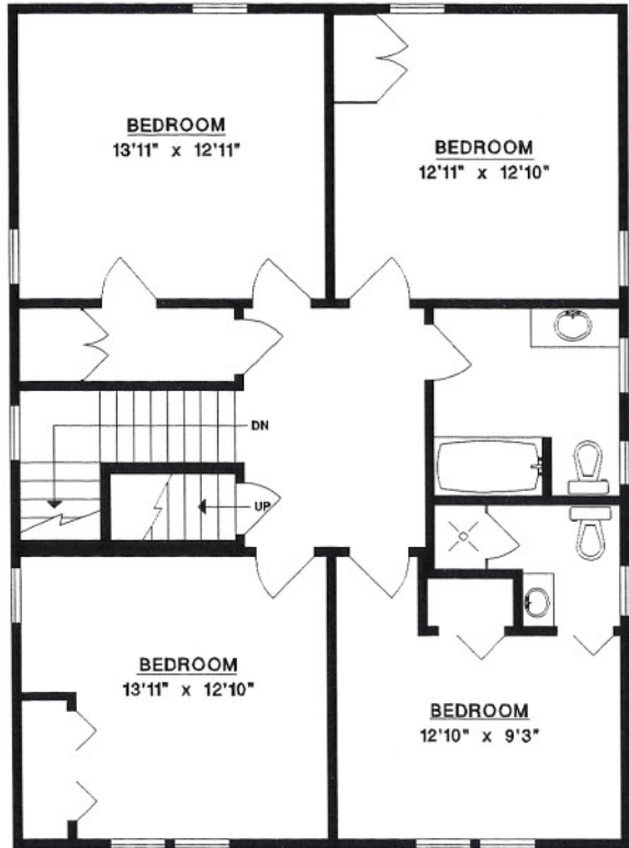
UPPER FLOOR
